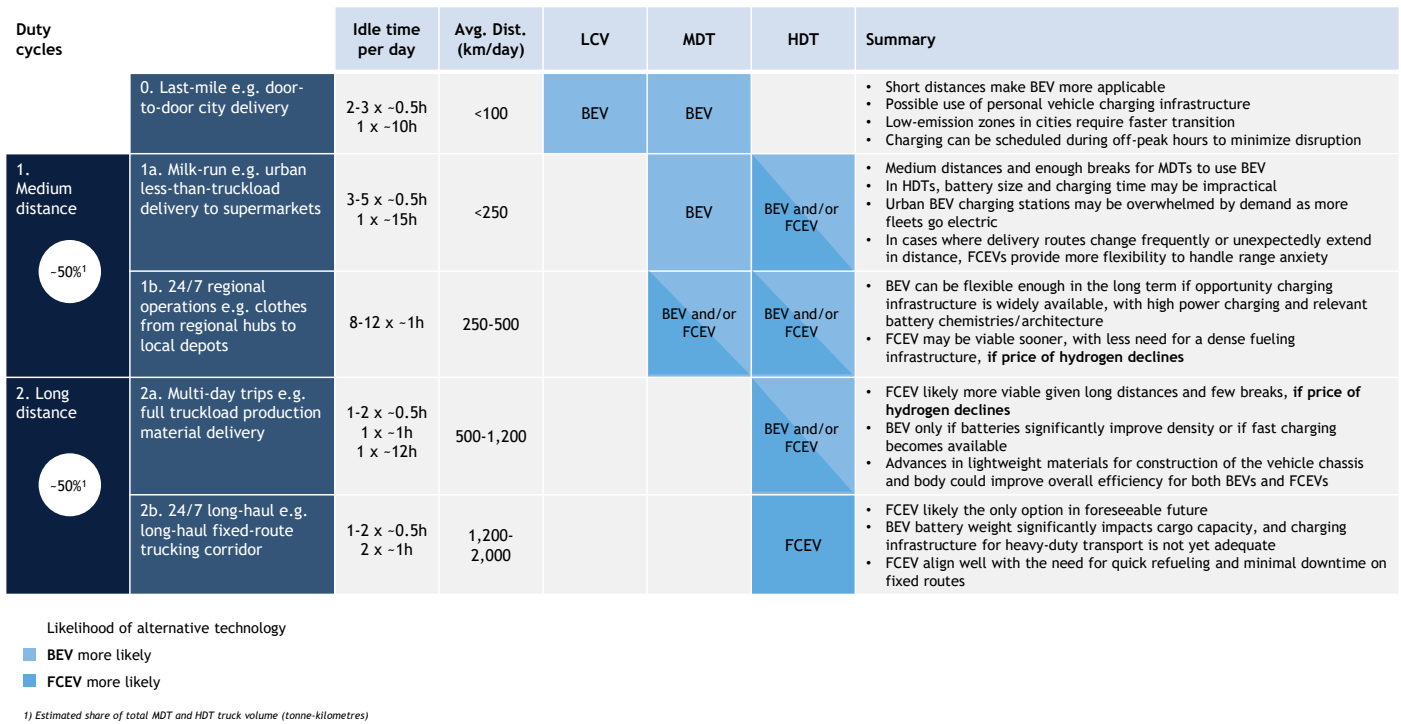
Figure 21 - Linking potential technologies to duty-cycles in ZE-M/HDV's
