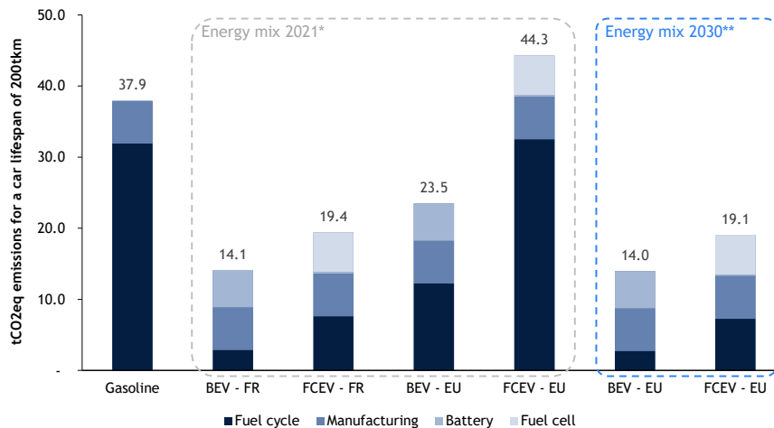
Figure 42 - GHG emissions per technology for 200tkm
