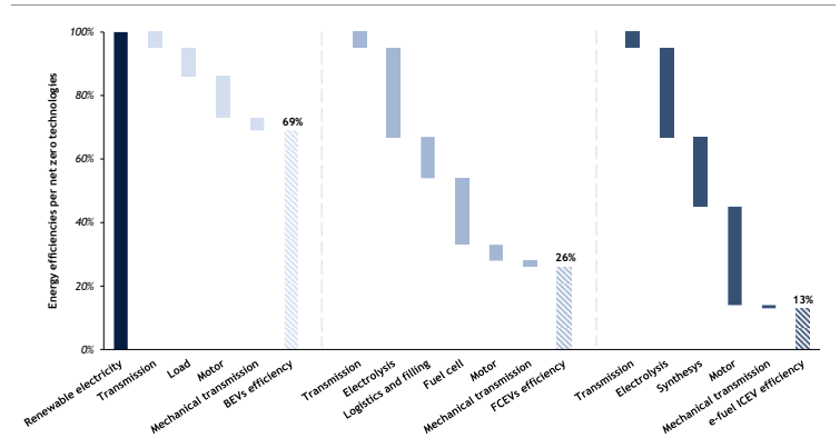
Figure 41 - Energy efficiencies of BEVs, FCEVs and ICEVs
